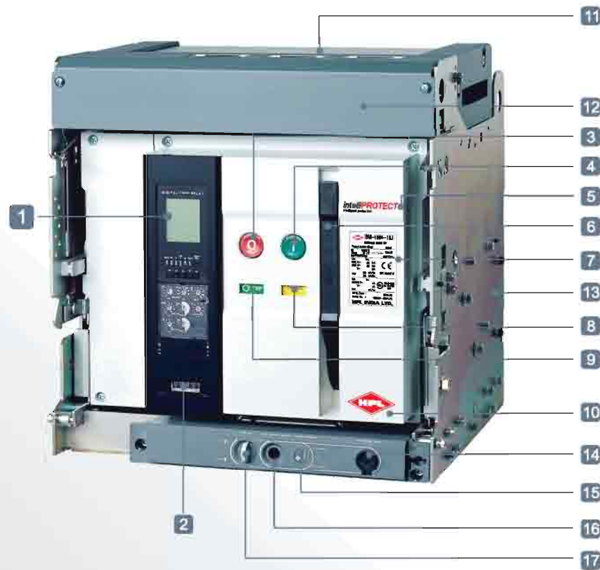
Draw-out ACB
